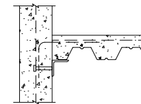
CONCRETE OR CMU WALL LEDGER DECK PARALLEL
