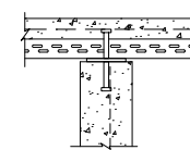
CONCRETE OR CMU WALL WITH EMBED PERPENDICULAR
