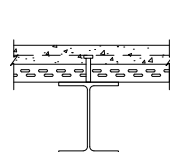
DECK PERPENDICULAR TO WIDE FLANGE BEAM
