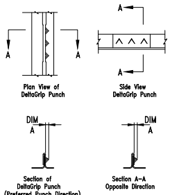
DELTA GRIP PUNCH VIEWS
