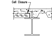
DECK TRANSITION ON WIDE FLANGE BEAM
