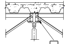
DECK ON OPEN WEB STEEL JOISTS AND OPEN WEB JOIST STEEL GIRDER
