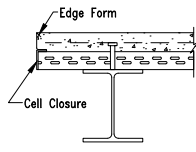
TWO PIECE EDGE FORM WITH DECK CANTILEVER ON WIDE FLANGE BEAM
