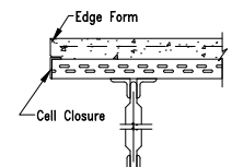
TWO PIECE EDGE FORM WITH DECK CANTILEVER OPEN WEB STEEL JOIST
